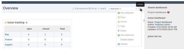
Fig. 5: Figure shows the project overview page and where to find the dashboard actions
